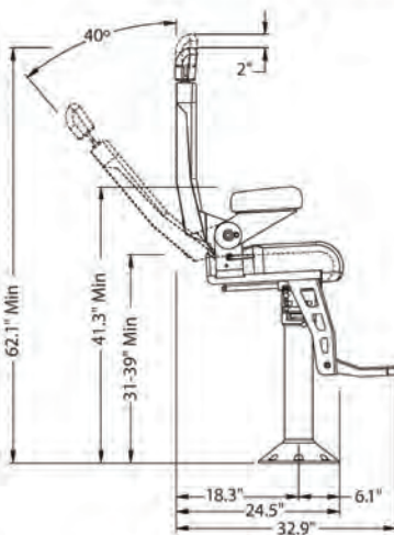
500NHX-1X2 & 500NH-1X2
